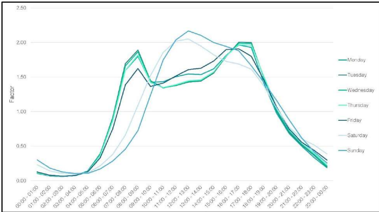
Figure 3 – Standard Diurnal Profile
