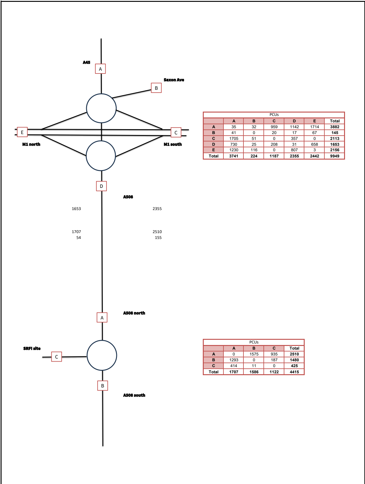
Diagram 7: 2031 total traffic flows - AM peak hour
