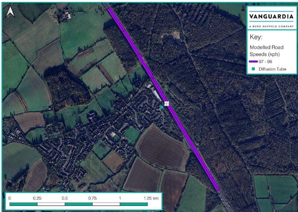
Figure D.2: 2023 Modelled Verification Road Network (M1 (Hartwell))
